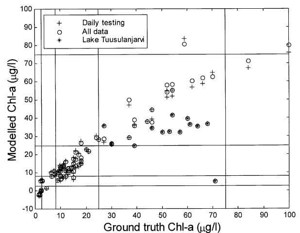
Fig. 6. Regression model for chl- a with AISA data. Vertical and horizontal lines represent quality class limits. Number of data points = 94. For all data, R^2 = 93.7\% ; for daily testing (separate training and testing data sets), R^2 = 91.9\% .
