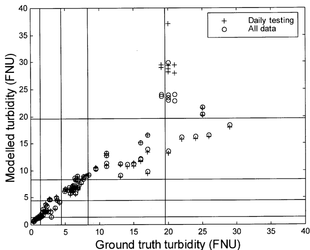
Fig. 5. Regression model for turbidity with AISA data. Vertical and horizontal lines represent quality class limits. Number of data points = 99. For all data, R^2 = 85.4\% ; for daily testing (separate training and testing data sets), R^2 = 76.1\% .
