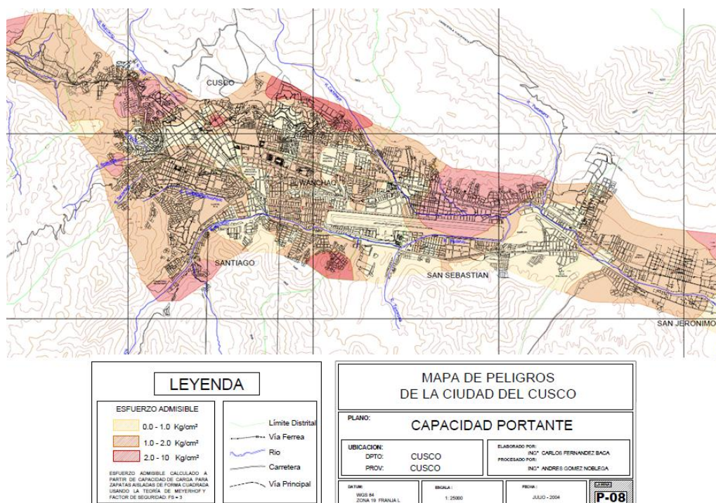
Figure 2.7 The bearing capacity ( \text{kg}/\text{cm}^2 ) of the soils for the city of Cusco. Source: adapted from Benavente Velasquez et al., 2004.
