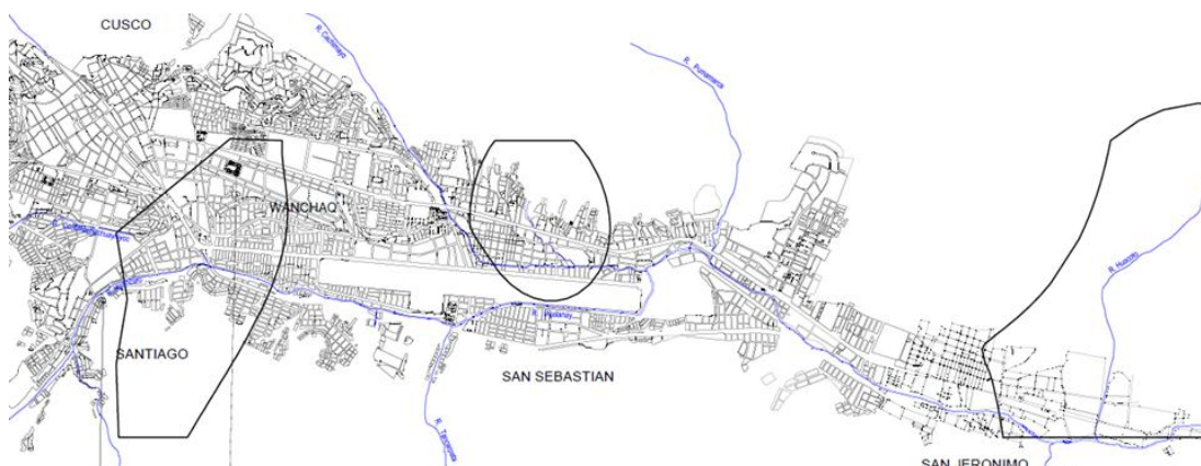
Figure 2.5 Outlines region considered susceptible to seismic activity for the city of Cusco and the surrounding districts, Source: adapted from Benavente Velasquez et al., 2004.
